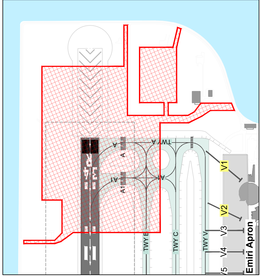
CONSTRUCTION BOUNDARY
